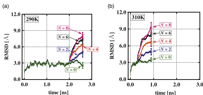
Fig. 7. (Color online) Root mean square deviation of DNA at 290 or 310 K. 2N hydrogen atoms are replaced with helium-3 atoms. The simulation time to stabilize the DNA structure for N = 0 structure is 2.0 ns or 0.3 ns for T = (a) 290 K or (b) 310 K, respectively. After the stabilization, we replace the N G bases to N T bases in the telomeric DNA. Then we run the MD simulation more for 0.6 ns at all temperatures.
