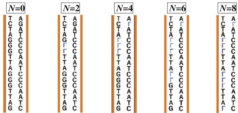
Fig. 4. (Color online) N guanines (G) in the original telomeric DNA is replaced with N replaced guanines ( \Gamma ). Two hydrogen atoms in each \Gamma are replaced with two helium-3 atoms as Fig. 2.
