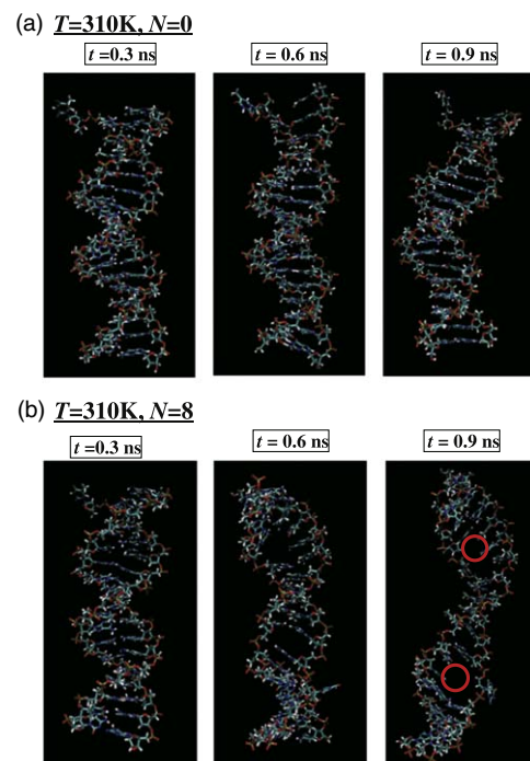
Fig. 6. (Color online) Time dependences of the DNA structures. (a) The structure of the non-substituted DNA, i.e. N = 0 case, has barely changed from the steady state t = 0.3 ns. (b) For N = 8 , the length between DNA chains becomes larger as time passes. Wide gaps between chains (the region denoted by circles) are found clearly at t = 0.9 ns. Some helium-3 atoms have flown away from the inside of DNA. The temperature is fixed to T = 310 K in both N .
