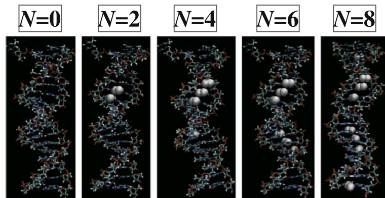
Fig. 5. (Color online) Initial molecular structures of the telomeric DNA for each N . The N = 0 structure was obtained by performing the MD simulation using NAMD code with CHARMM36 potential, Langevin thermostat algorithm and the Nosé–Hoover piston method until the structure becomes stable. The 2N hydrogen atoms are replaced to helium-3 atoms (gray balls). The charge distribution in a guanine of the telomeric DNA is also caused by loss of hydrogen atoms. The charge distribution in the replaced guanine \Gamma is given by DFT code as in Table I. Using these initial structures, we perform the MD simulation and obtain the structure transformation of DNA. These snapshots corresponds to the case of T = 310 K.
