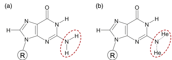
Fig. 2. (Color online) (a) The original guanine (G) structure. The two hydrogen atoms of guanine are replaced by two helium-3 atoms as shown in (b). The replaced guanine is named as \Gamma . Though the hydrogen-nitrogen bond in the original guanine (G) is a covalent bond, the helium-3 and the nitrogen interact with each other not by a covalent bond anymore, but by a weak interaction, i.e. an intermolecular force.
