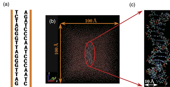
Fig. 1. (Color online) (a) The base sequence of the DNA. (b) A telomere structure of human DNA with 71 000 water molecules, 121 \text{Na}^+ and 89 \text{Cl}^- . The DNA is composed of 1078 atoms. The initial simulation box is 100 \text{ \AA} \times 100 \text{ \AA} \times 100 \text{ \AA} . (c) The original configuration of the telomeric DNA.
