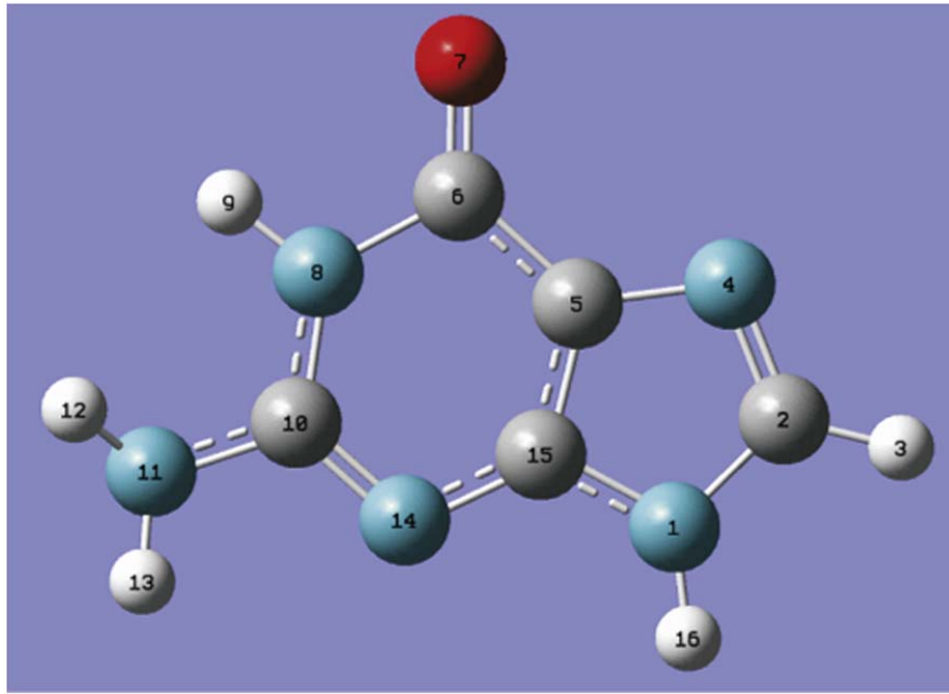
Fig. 3. (Color online) Molecular structure of guanine optimized by DFT calculation. The integers denote the indices of the atoms. Red, blue, light-gray and dark-gray balls denote oxygen, nitrogen, hydrogen, and carbon, respectively. Charge distribution is given in Table I.
