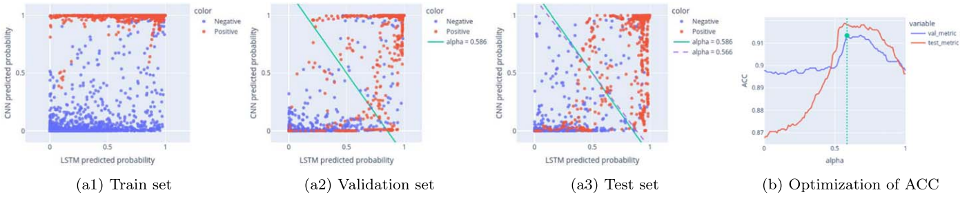
Figure 11. (a1)–(a3): CNN predicted probability (y-axis) vs. LSTM predicted probability (x-axis) for the train, the validation, and the test set. The green solid lines in (a2) and (a3) show the decision boundary of the ensemble with meta-learner fitted on the validation set. The violet dashed line in (a3) is analogous to the green lines except that it is fitted on the test set, and hence can be seen as the oracle. (b): ACC as a function of \alpha on the validation and the test set. The vertical green line shows the value of \alpha that maximizes the validation ACC. The leftmost values of the ACC curves ( \alpha = 0 ) correspond to the ACC of the CNN, and the rightmost values of these curves ( \alpha = 1 ) correspond to the ACC of the LSTM.
