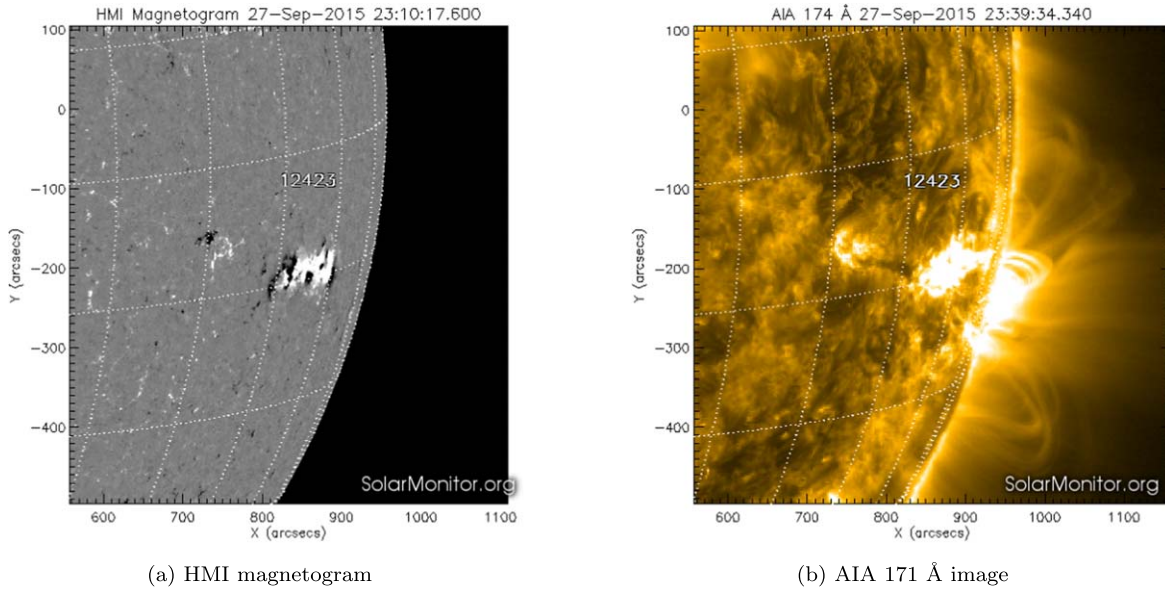
Figure 16. Line-of-sight magnetic field (panel (a)) and solar EUV image (panel (b)) of HARP 5982 (NOAA AR 12423) at 23:10:17 on 2015 September 27. Images are taken from https://solarmonitor.org/ . Note that the image title of panel (b) should be “AIA 171 Å” instead of “AIA 174 Å.”
