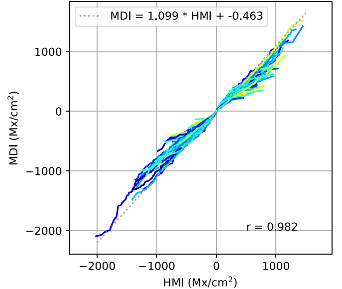
Figure 1. Q – Q (quantile–quantile) plot of 50 matched magnetogram pairs of HARP and TARP from 2010 May 1 to October 28. Active regions with pixels outside of \pm 70^\circ from the central meridian are not used. For each pair, the cotemporal magnetograms are sampled at a rate of every 8 hr. The pixels within the intersection of the bounding boxes of active region pairs are used. Lighter colors indicate higher latitudes.
