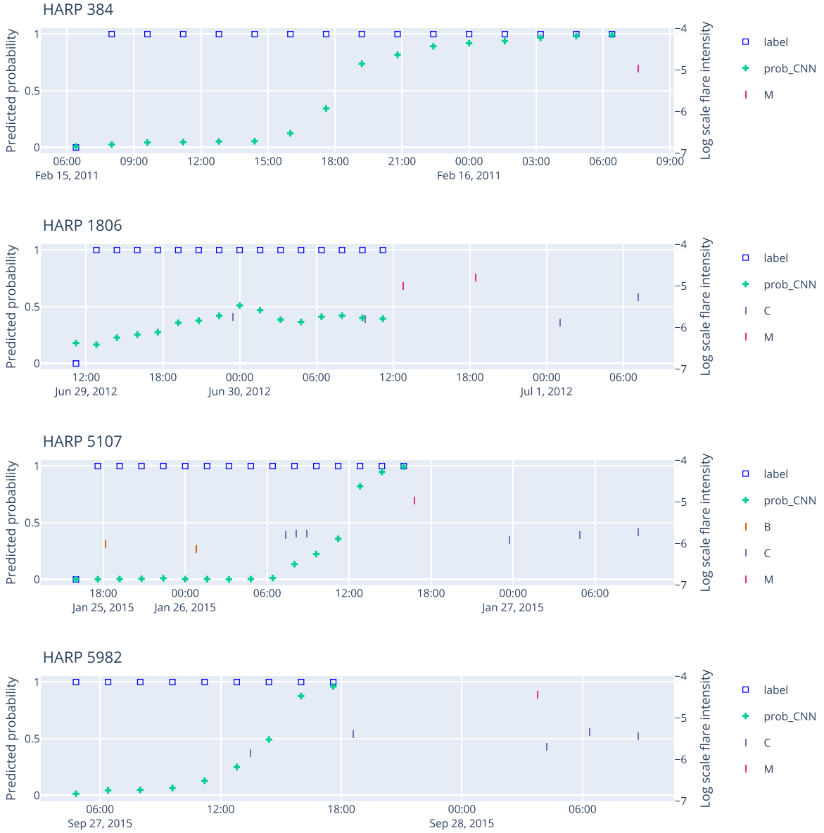
Figure 13. CNN predictions of part of the time series of in HARP 384, 1806, 5107, and 5982. The labels are shown as blue open boxes and the predicted probabilities are shown as green plus symbols. The point-in-time instance is labeled as positive if an M1.0+ flare occurred in the succeeding 24 hr in that active region. GOES flare events during and 24 hr within the sample sequence are shown as short vertical bars, with y-coordinates indicating flare intensities (peak flux in \text{W m}^{-2} ) on a log scale.
