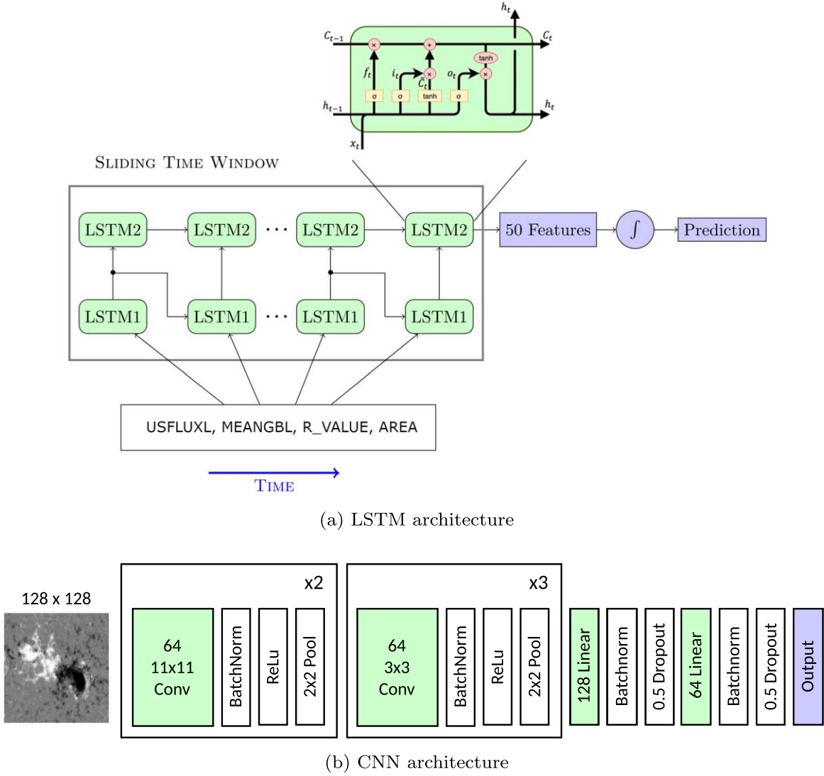
Figure 4. Neural network architectures. Panel (a) shows the LSTM architecture. Panel (b) shows the CNN architecture.
