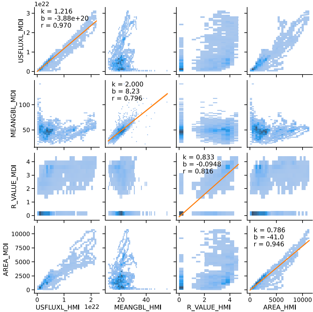
Figure 2. Two-dimensional histograms of summary parameters USFLUXL , MEANGBL , R_VALUE , and AREA between SHARP and SMARP. SHARP summary parameters are suffixed with _HMI and SMARP with _MDI . The orange lines in the diagonal blocks are the least-squares fit of SMARP summary parameters on the corresponding SHARP summary parameters, with coefficient k , intercept b , and Pearson correlation coefficient r displayed in the corner.
