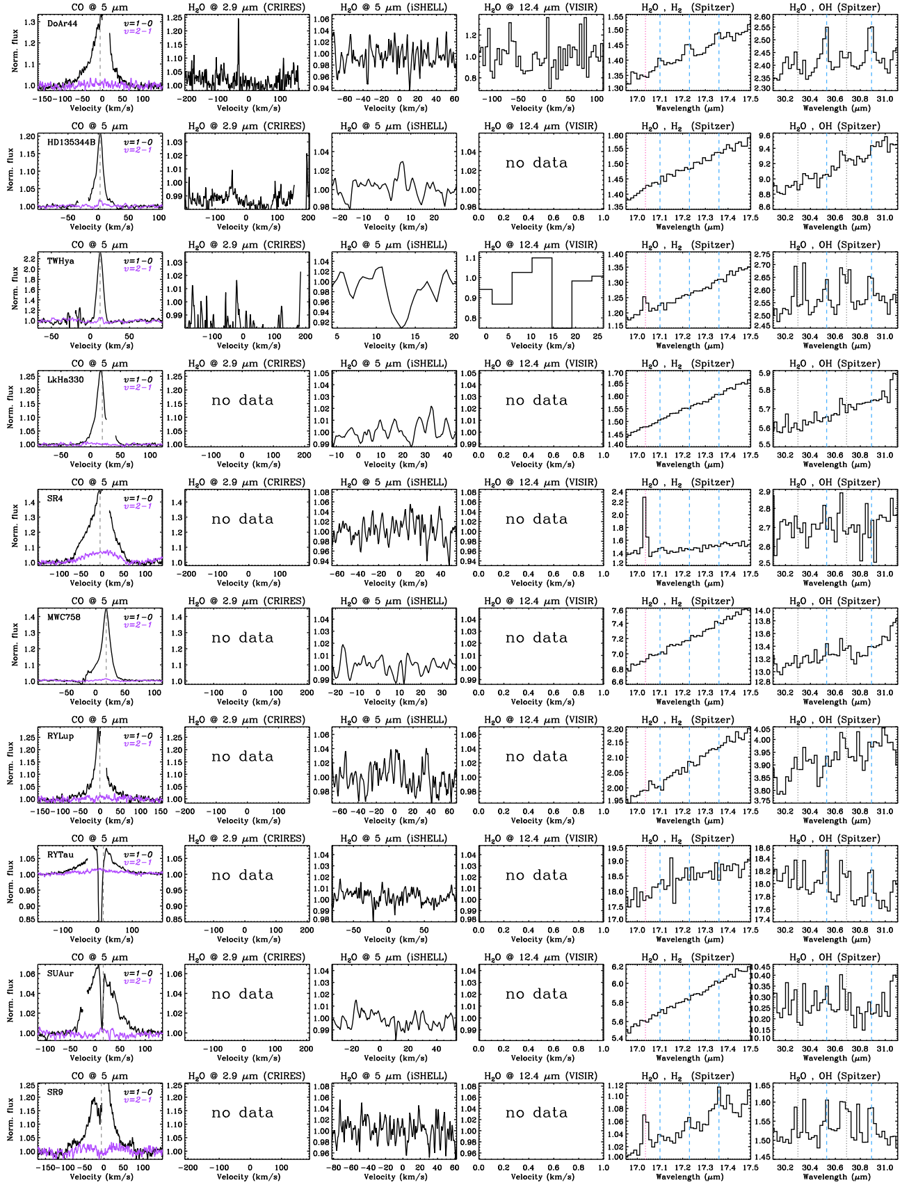
Figure 19. Same as Figure 16, for disks with inner dust cavities.
