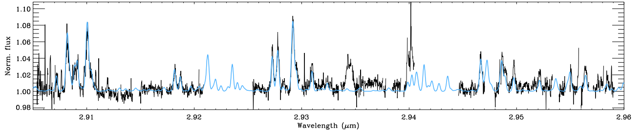
Figure 2. Example of a CRIRES L -band spectrum, for the disk of DR Tau (from Banzatti et al. 2017). A water emission spectrum is shown in light blue, using the LTE slab model fit described in Section 4.4. The prominent feature near 2.935 \mu\text{m} is an OH doublet.
