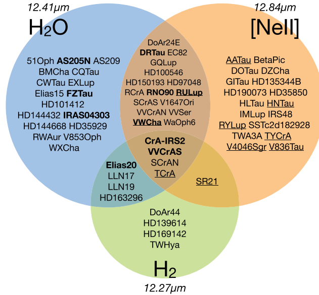
Figure 23. Venn diagram showing spectral settings and sample obtained in the VISIR survey included in this work. Detections are shown in boldface for water (presented in this work), and underlined for [Ne II] (presented in Pascucci et al. 2020). No detections are reported for H 2 .
