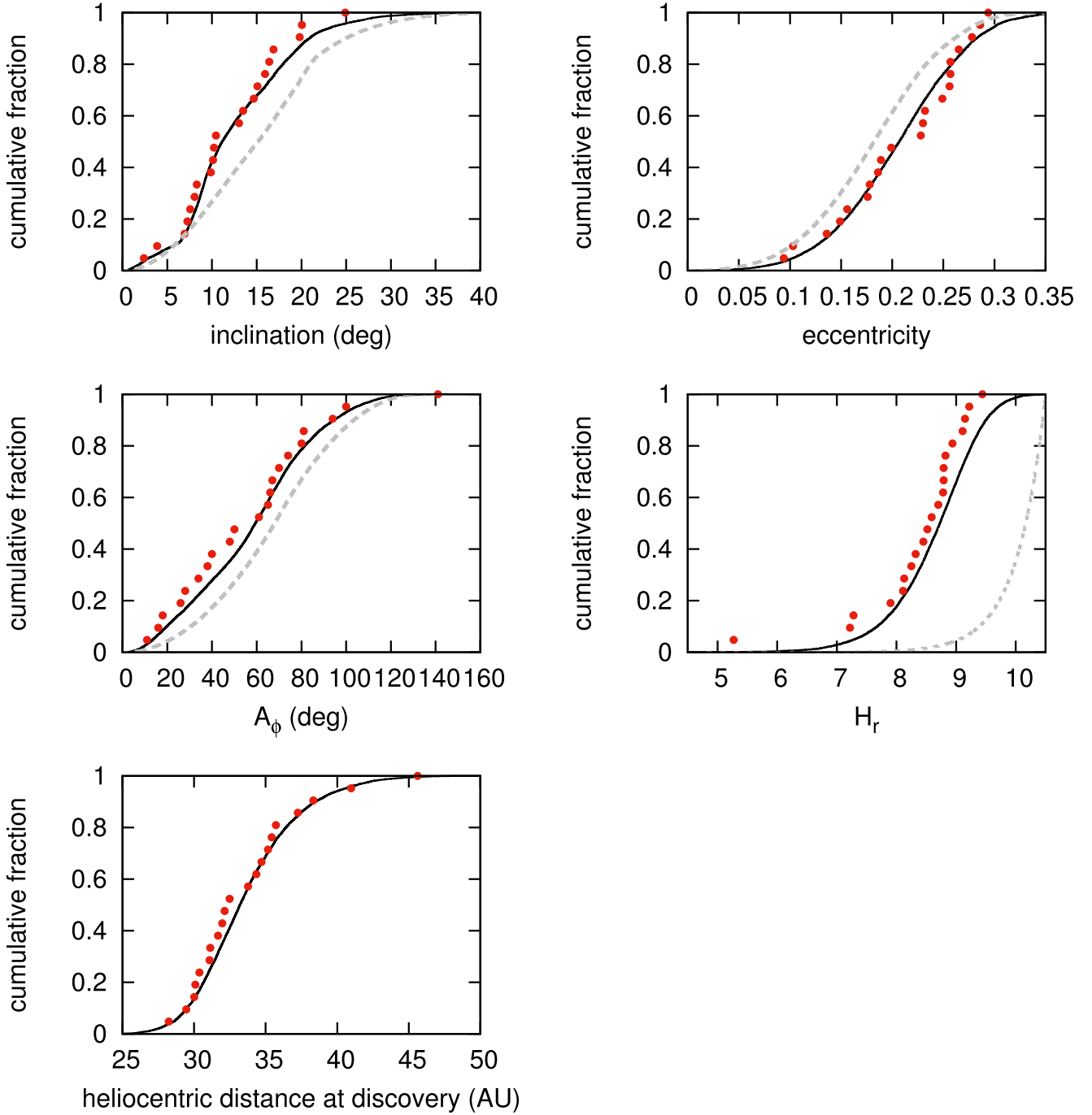
Figure 6. Cumulative one-dimensional distributions in i , e , A_\phi , H_r , and distance at discovery for the observed 13AO and 13AE block plutinos (red dots), the intrinsic plutino population for our nominal plutino model (gray dashed lines), and for the synthetic detections from our nominal plutino model (black lines). The differences between the intrinsic models and the synthetic detections show the effects of the observational biases.
