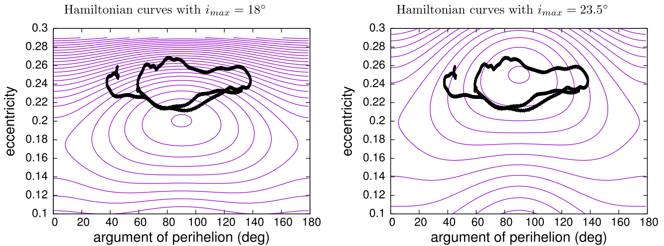
Figure 18. Evolution of plutino o3o08 (black dots) from a numerical simulation that includes the Sun and the four outer planets plotted over approximate Hamiltonian level curves for i_{\max} = 18^\circ (left panel) and i_{\max} = 23.5^\circ (right panel). The object has i_{\max} = 18^\circ , but the poor match in the left panel indicates that the expression for the approximate Hamiltonian in the three-body problem as given by Wan & Huang (2007) is not a good match to the dynamics in the full integrations.
