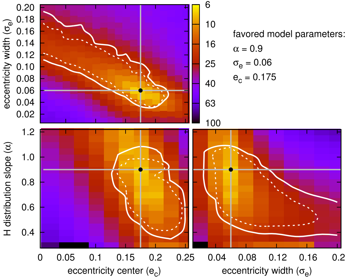
Figure 4. Color maps: goodness-of-fit for various plutino model parameters as measured by a summed \chi^2 statistic for the e , H , and d distributions. White lines: rejected parameter values using the summed AD statistic for the e , H , and d distributions at the 99% confidence level (solid white curves) and the 95% confidence level (dashed white curves). Our favored model parameters (based on minimizing the summed \chi^2 statistic) are shown by the black dots. Each panel is a two-dimensional cut in our three-dimensional parameter space search. For each panel, we fix one parameter at its favored value and show the goodness-of-fit map for the other two parameters (for example, in the top panel, \alpha is fixed at 0.9 to show the allowed range in \sigma_e and e_c for that value of \alpha ).
