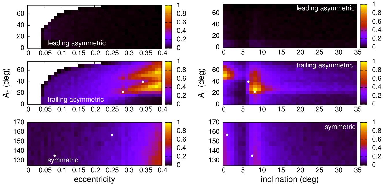
Figure 9. Relative visibility (color coded) of e - A_\phi and i - A_\phi 2:1 phase space for the OSSOS 13AO and 13AE blocks assuming an even split between the leading asymmetric, trailing asymmetric, and symmetric libration centers as well as uniform e , i , and A_\phi distributions within the resonant phase space of all three libration islands. The white dots show the OSSOS detections.
