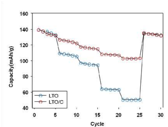
Fig 2 Discharge capacity by current density of LTO and LTO-C composite from styrene in \text{LiBF}_4/\text{PC}
