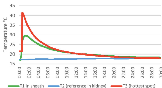
Figure 6. Representative graph of temperatures measured from baseline reference at opposite pole of kidney (blue) just within the tip of the sheath (green), and from the hottest location identified by infrared imaging (red, accounting for the higher initial temperature). Injection began at 10 s and lasted for 6 s, sampling at 1 Hz. The temperature rose abruptly with the peak at 25^\circ\text{C} above the baseline and gradually decayed over the 30 min duration of the experiment. Peak temperature deep in the tissue is much higher than indicated on the surface by infrared imaging and also higher than at the sheath tip.
