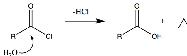
Figure 4. Aqueous hydrolysis reaction of an acid chloride as predicted in thermoembolization with water as the dominant nucleophile. Note the generation of two acidic protons from formation of the parent carboxylic acid and loss of HCl, as well as the release of substantial heat energy ( -93 \text{ kJ/Mole} ).
