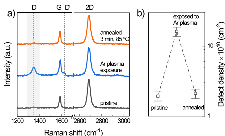
Figure 3. Reversibility of plasma-induced defects upon in situ annealing. (a) Evolution of Raman spectra of graphene. A defect mode appears in pristine graphene (black) upon plasma exposure (blue). After in situ annealing to 85 °C the mode disappears (red). (b) The defect density extracted for each step in (a).
