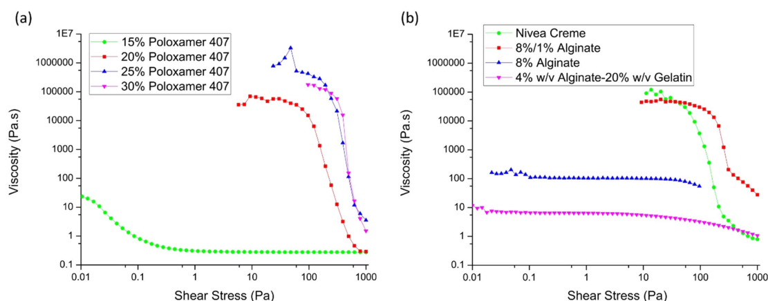
Figure 4. Shear stress ramp data for all experimental samples, performed at 24^\circ\text{C} for all samples except the alginate-gelatin (4% w/v alginate hydrogel, 20% w/v gelatin) which was measured at 37^\circ\text{C} .
