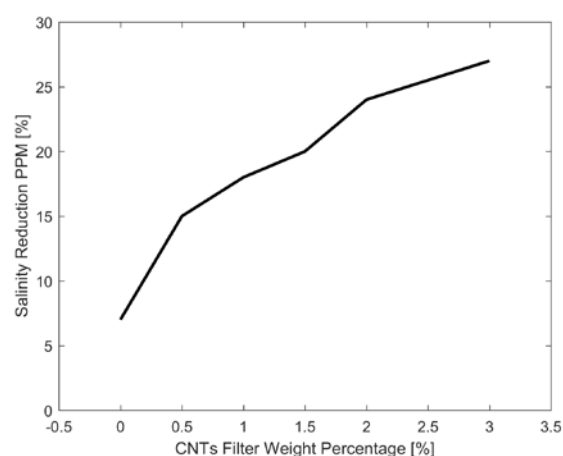
Figure 10. Effect of CNTs Weight on Reduction Percentage of Dissolved Salts for Red Sea Water PPM%.
