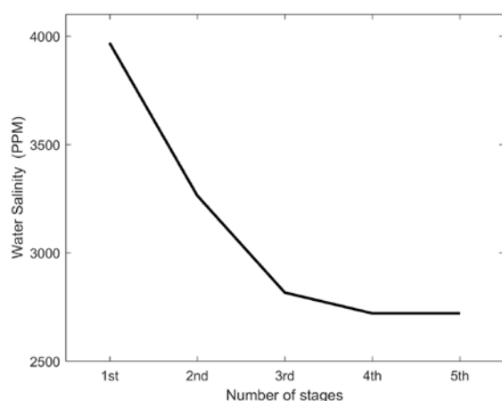
Figure 15. Effect of Filtration Stages at 3% wt. filter on Dissolved Salts for Brackish Water.
