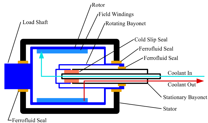
Figure 2. Coolant transfer coupling concept.
