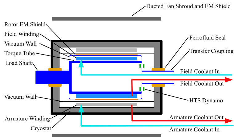
Figure 1. Superconducting motor concept with HTS field winding.
