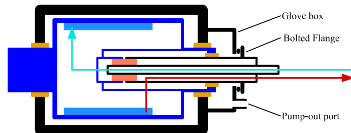
Figure 3. Leak-free coolant transfer coupling concept
