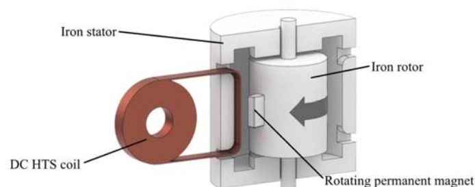
Figure 5. Brushless HTS dynamo concept.
