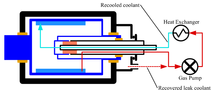
Figure 4. Rotor cooling system with stationary cooler
