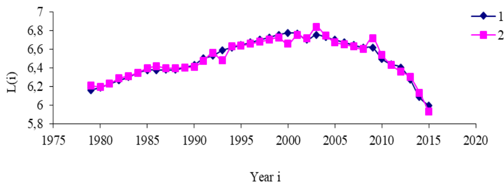
Figure 1. Field data (1) and model calculations (2) of deer abundance in the Taimyr-Evenki population.
