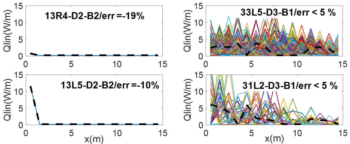
Figure 3. Potential heat load profiles after beam dump 6737 (high beam intensity - 6.5\text{ TeV} )
