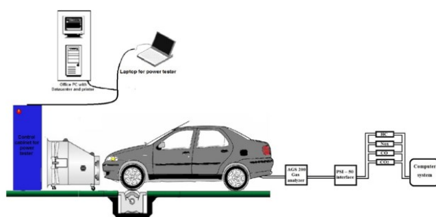
Figure 14. Chassis test bench.
