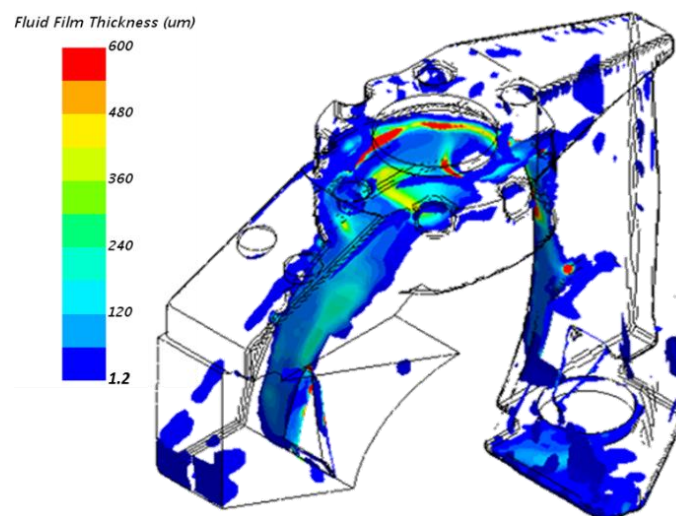
Figure 6. Oil film on the inlet distributor walls (0.4 s).
