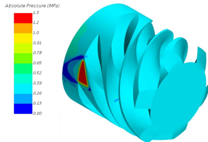
Figure 10. Pressure field on the single screw expander.
