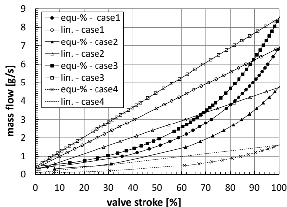
Figure 4. Calculated valve characteristics for compressible flow.
