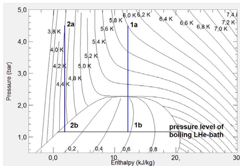
Figure 3. Comparison of two options for liquefaction into LHe-bath.
