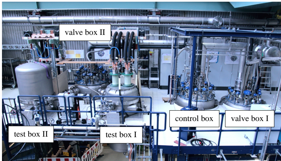
Figure 1. Photo of the Current Lead Test Facility Karlsruhe.
