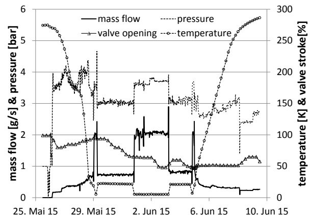
Figure 5. Measured data of a control valve with K_{vs} = 0.16 .
