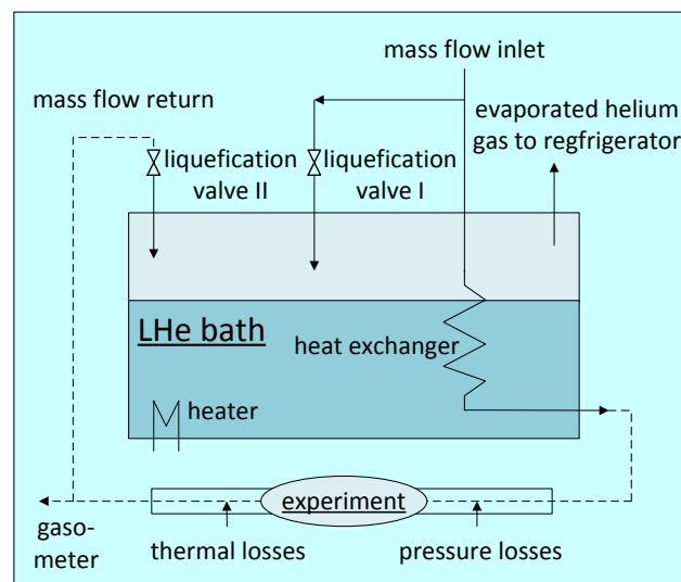
Figure 2. Flow scheme of the LHe-bath with its cooled HEX.
