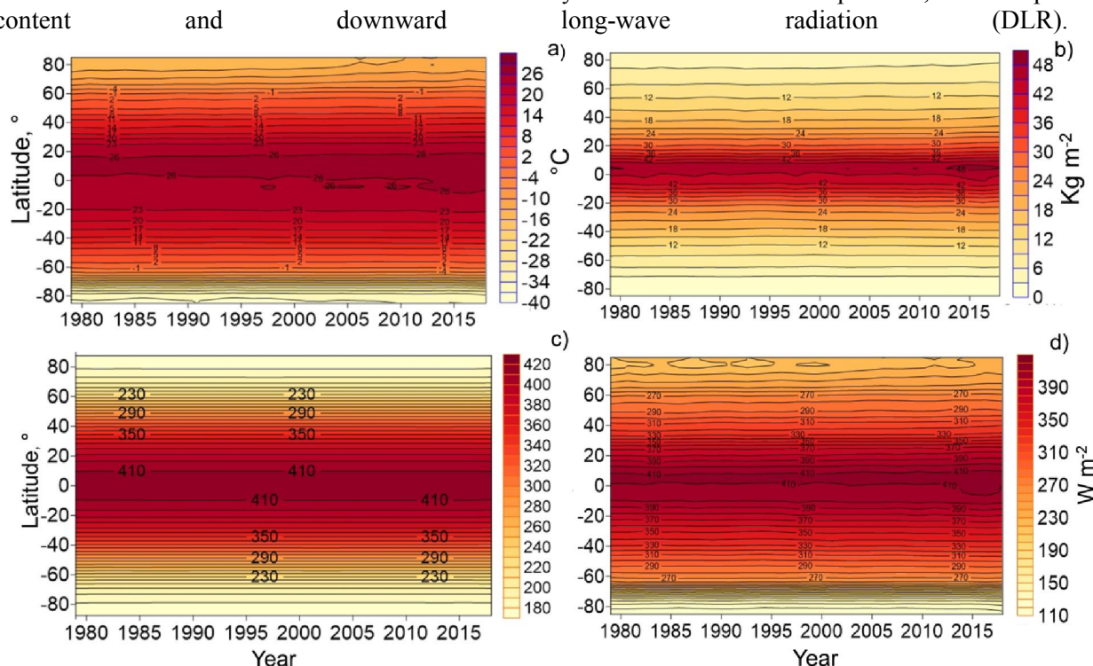
Figure 5. Zonal values of mean annual atmospheric parameters.
