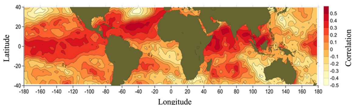
Figure 3. Correlation between SST anomalies in 40°S–40°N zone in October and anomalies of the meridional atmospheric transport of sensible heat in December–February through the Atlantic gate in 70°N on 27 months later for 1982–2015.
