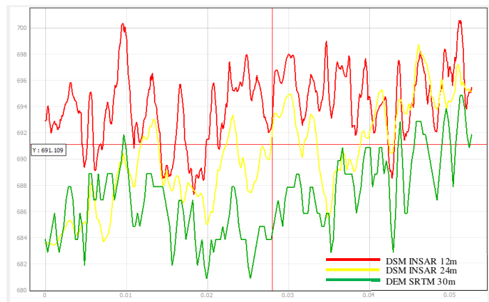
Figure 15. Trend of Plotting Profiles on DSM in Flat Area
