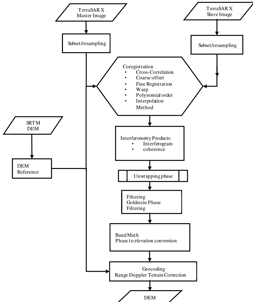
Figure 4. Flowchart of SAR Image Processing.
