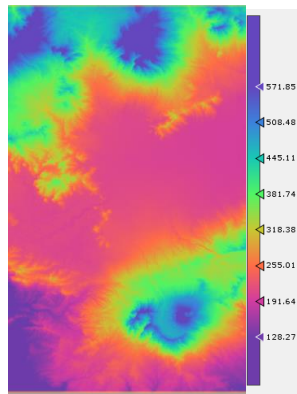
Figure 8. Topo phase
