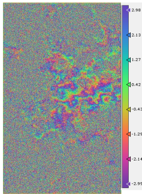
Figure 7. Interferogram
