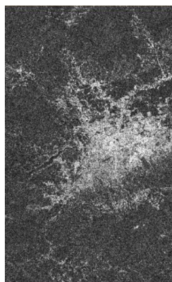
Figure 6. Coherence
