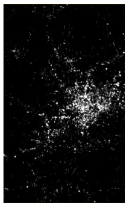
Figure 5. Intensity
