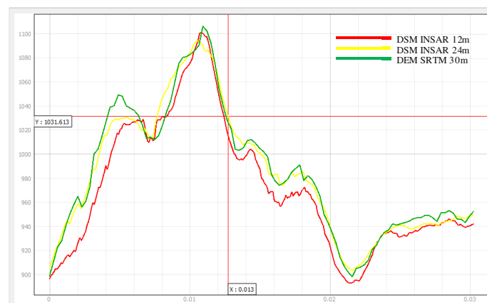
Figure 13. Trend of Plotting Profiles on DEM in Higher Regions
