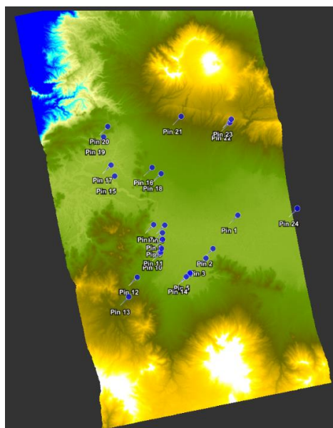
Figure 10. DEM Looking with Ground Control Points Using GPS
