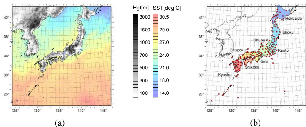
Figure 1. Modelling domains showing (a) topography of land areas and average sea surface temperature of August 2014; (b) locations of meteorological observatories and division of regions for analyses of precipitation.
