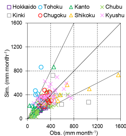
Figure 3. Scatter plots of monthly precipitation at the meteorological observatories in August 2014 for the observation and the simulation results in the baseline condition. The plots are classified as each region.
