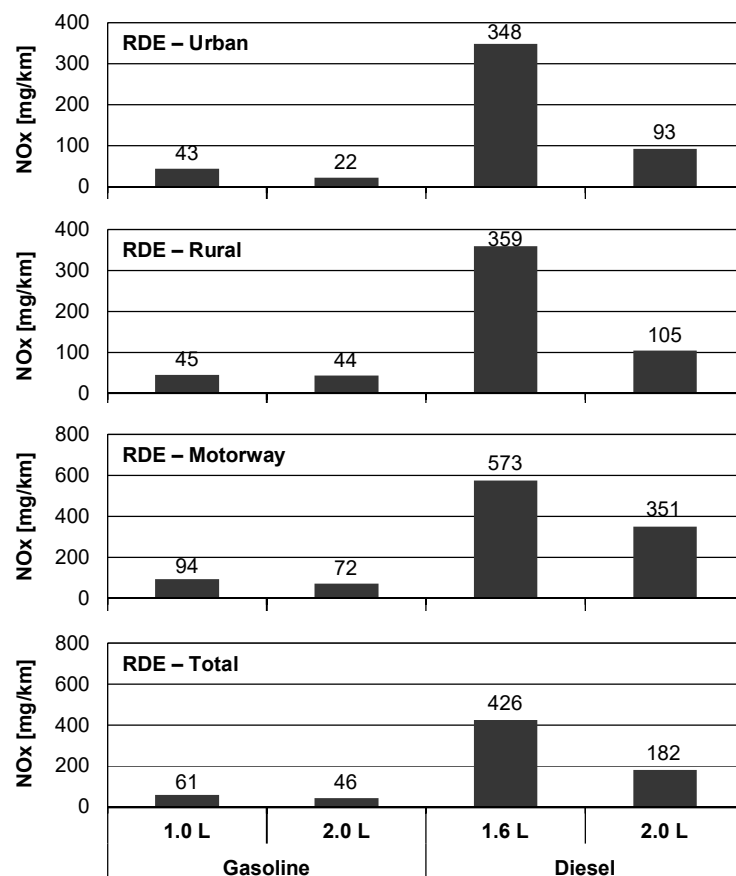
Figure 7. Combined results of the nitrogen oxides emission of the tested vehicles with Gasoline engines (1.0 L, 2.0 L) and with Diesel engines (1.6 L, 2.0 L) in individual sections of the RDE test.
