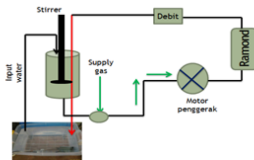
Figure 1. Working scheme of the nanobubble device.
