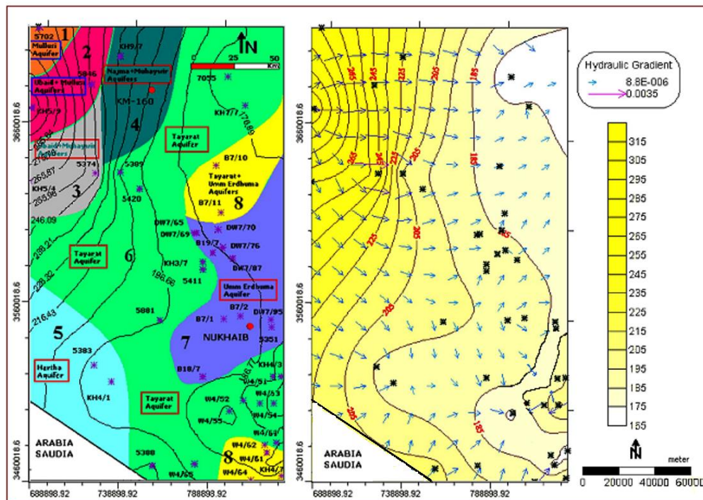
Fig. 17. Groundwater flows within the study area.
