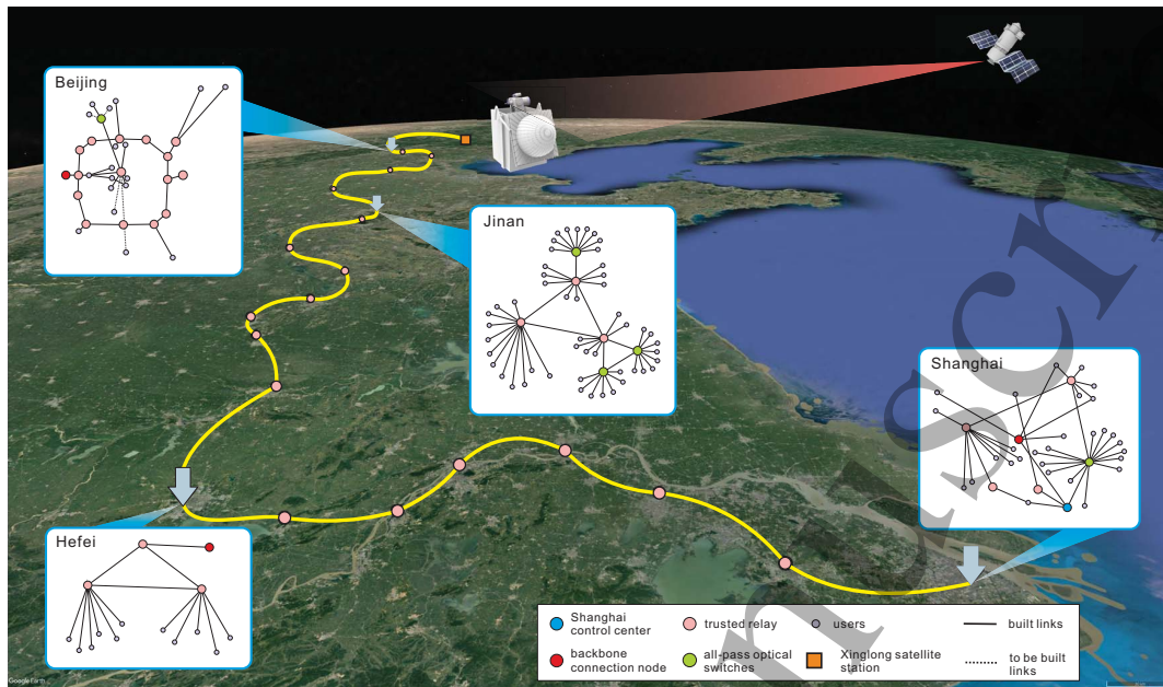
Figure 21. The Beijing-Shanghai backbone network connects four metropolitan area QKD networks and also features a long distance quantum satellite link covering 2600 km between Xinglong and Nanshan (not shown). Reprinted figure with permission from [420]. Copyright 2020 by the American Physical Society.
