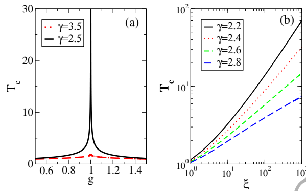
Figure 4. Behavior of the critical temperature T_c as the expected degree distribution of Eq. (4) is varied in an annealed random transverse field Ising model with random onsite energies modelling the superconductor-insulator phase transition on a complex network. Left: external parameter g controls the transition to a pure power-law via \xi \propto |g/g_c - 1|^{-1} , where here we take g_c = 1 . Right: \xi is varied directly. Reprinted figure with permission from [94]. Copyright 2012 by the American Physical Society.
