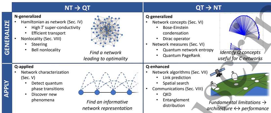
Figure 1. We distinguish between four distinct research lines on complex quantum networks: network-generalized, quantum-applied, quantum-generalized and quantum-enhanced. Here these research lines are schematically presented with a figure and with illustrative research questions. These different research lines will be presented in the indicated Sections.
