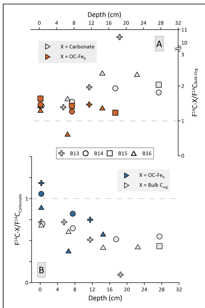
Figure 3. Comparison of fraction modern values ( F^{14}C ) between carbon phases measured at the same sediment depth for each station. (A) F^{14}C of benthic foraminifera (carbonate) and F^{14}C of OC associated to reactive iron (equation (1)), OC-Fe R , relative to the F^{14}C values of bulk organic carbon. Values >1 are younger ( ^{14}C -enriched) than the bulk organic matter. (B) F^{14}C values of OC-Fe R and bulk organic carbon relative to the F^{14}C of carbonate. Values <1 show older ( ^{14}C -depleted) signatures compared to the benthic foraminifera phase.
