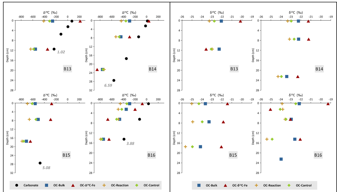
Figure 2. Downcore \Delta^{14}\text{C}_{\text{org}} (left) and \delta^{13}\text{C}_{\text{org}} (right) values in the sediment residuals of the control and extraction experiment and bulk sediment. These are shown relative to the \Delta^{14}\text{C} content of benthic foraminifera (carbonate). The isotopic signatures of the organic carbon fraction bond to \text{Fe}_\text{R} ( \Delta^{14}\text{C}\text{-Fe}_\text{R} and \delta^{13}\text{C}\text{-Fe}_\text{R} ) are calculated by mass balance (equations (1) and (2)). Grey numbers indicate uncalibrated radiocarbon dates of the lowest biogenic carbonate measurement in kyr BP.
