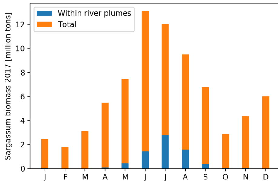
Figure 4. Monthly mean Sargassum biomass for year 2017 estimated from MODIS in the Caribbean and Central Atlantic ( 5^{\circ} S– 25^{\circ} N, 89^{\circ} W– 15^{\circ} E). The blue bar marks the fraction of the biomass which is colocalized with the model river plume (defined as areas with surface concentration of riverine waters >0.05 , i.e. more than 5% of kg of water with riverine origin per kg of ocean water; the spatial distribution of the river tracer is shown in figure 3(c)).
