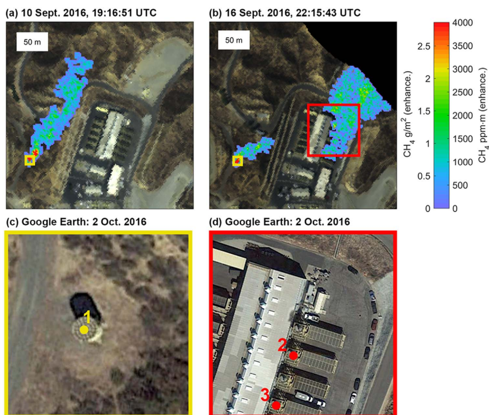
Figure 5. Attribution of multiple methane emission sources detected at Honor Rancho. (a) AVIRIS-NG result shows a persistent methane plume for source 1 (yellow box in (a) and (c)). (b) Source 2 and/or source 3 appeared episodically (red box) for 29% of flights. (c) Close-up of source 1 with high-resolution satellite imagery (Google Earth). The facility operator confirmed that source 1 is the facility's emergency shut down stack—likely due to a leaking isolation valve. (d) Close-up of sources 2 and 3—likely from the rod pack vents for reciprocating compressor units 2 and 4.
