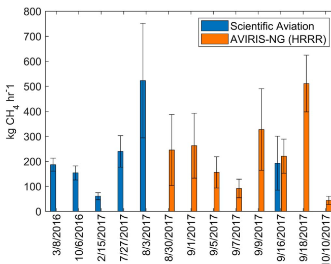
Figure 4. Estimated methane emissions for the Aliso Canyon UGS facility following return to operations using Scientific Aviation in situ estimates (blue) and AVIRIS-NG estimates using the mass balance method with HRRR wind speeds (orange). On 9/16/2017, methane emissions were estimated at 193 \pm 108 \text{ kg h}^{-1} for Scientific Aviation compared to 221 \pm 68 \text{ kg h}^{-1} using AVIRIS-NG and HRRR winds.
