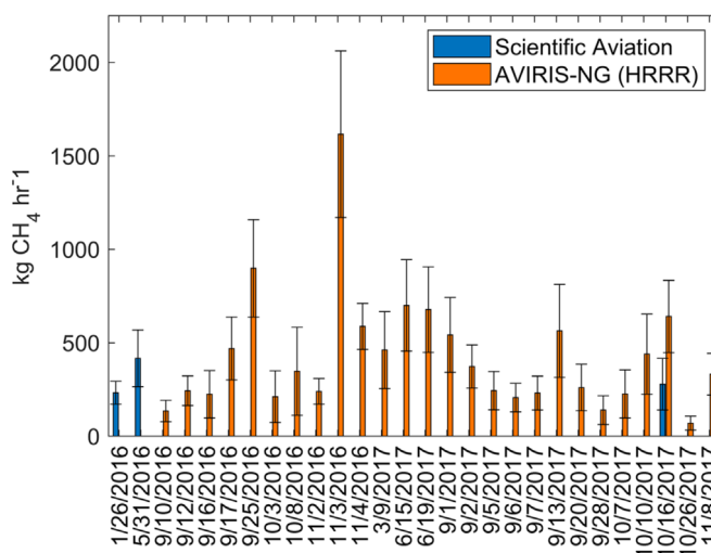
Figure 6. Estimated methane emissions for the Honor Rancho UGS facility using Scientific Aviation in situ estimates (blue) and AVIRIS-NG estimates using the mass balance method with HRRR wind speeds (orange).
