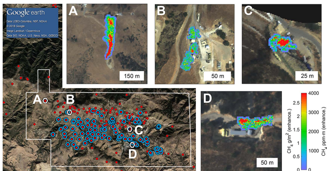
Figure 3. Characterizing methane emissions from Aliso Canyon following return to operations. Aliso Canyon field spans roughly 14 km 2 and records (Division of Oil, Gas, and Geothermal Resources DOGGR 2018) indicate 251 wells (red dots)—115 of which are linked to the gas storage reservoir (blue circles) and the rest connected to shallower oil-producing formations (combination of active, idle, and plugged wells). Subpanels (a) through (d) indicate methane plumes observed with AVIRIS-NG overlain on true color imagery that correspond to the locations shown in the map of the Aliso Canyon field from an oil well (a), tank (b), drill rig (c), and shutdown stack near the storage facility's compressor station (d).
