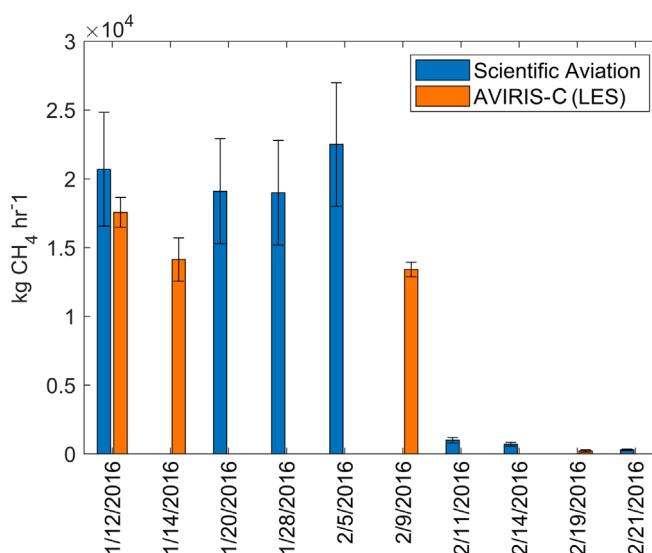
Figure 1. Time series of Aliso Canyon methane emissions for January–February 2016 comparing independent estimates from contemporaneous Scientific Aviation in situ estimates (blue) and AVIRIS-C remote sensing combined with LES modeling (orange). Emission estimates derived with AVIRIS-C are shown as daily averages. Both AVIRIS-C and Scientific Aviation capture the step function reduction in emissions following the February 11, 2016 bottom kill of the leaking well and subsequent slow decay from soil outgassing.
