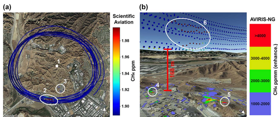
Figure 7. Results from Scientific Aviation and AVIRIS-NG surveys of Honor Rancho on October 16, 2017. (a) Location 1 denotes the center of the cylindrical flight path of Scientific Aviation and location 2 indicates regions where higher in situ methane concentrations were observed. Two AVIRIS-NG \text{CH}_4 plumes were observed at location 3 with plume shapes and Scientific Aviation enhancements consistent with local winds towards the southwest. (b) Perspective view showing AVIRIS-NG \text{CH}_4 plumes at location 3 overlaid on terrain for an unknown source (location 4) and an emergency shutdown stack (location 5). The lowest altitude Scientific Aviation flight paths were around 168 m above the main facility hence only enhancements at greater than 168 m above the ground were measured (location 6).
