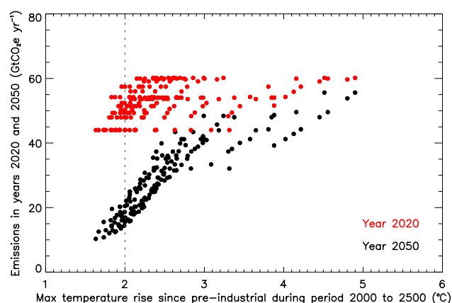
Figure 2. Emissions in years 2020 (red dots) and 2050 (black dots) for each core emission trajectory with zero or low floors. This is plotted against the median in maximum temperature rise in period 2000–2500, derived from the probabilistic ensembles for each core trajectory. The vertical dashed line corresponds to 2 °C global warming.
