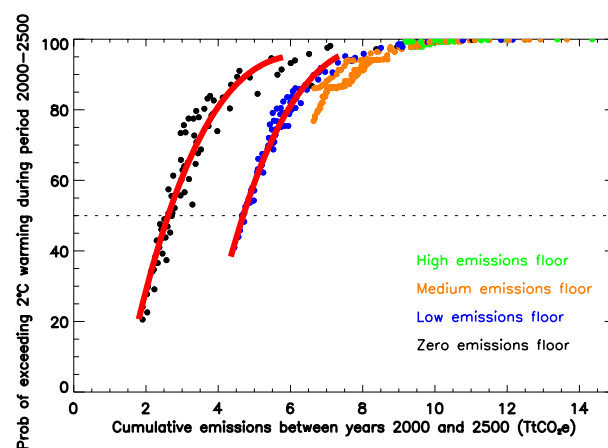
Figure 3. The probability of exceeding 2 °C of global warming since pre-industrial times at any point during the period 2000–2500, as a function of cumulative emissions between years 2000 and 2500 (in units of trillion i.e. 10 12 tonnes of CO 2 e). This is for the core emissions profiles. The different colours distinguish the long-term emissions floors, high (16 GtCO 2 e yr -1 ), medium (11 GtCO 2 e yr -1 ), low (6 GtCO 2 e yr -1 ) and zero (0 GtCO 2 e yr -1 ). The red line is the curve of best fit for the low and zero floors. (Additional available core emission scenarios following a B2 SRES baseline emissions scenario were also included). The 50% probability of staying below the 2 °C threshold is marked as the dashed line.
