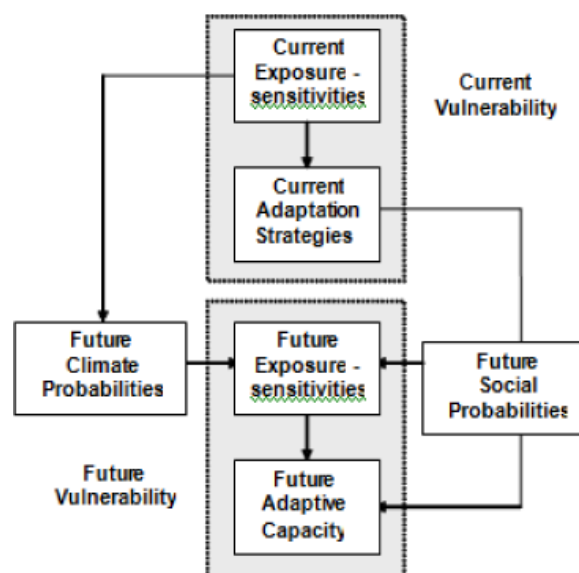
Figure 4. Two step analytical framework use to structure the empirical assessment of what we know and do not know about climate change vulnerability (after Ford and Smit 2004, Smit and Wandel 2006, Ford et al 2008).
