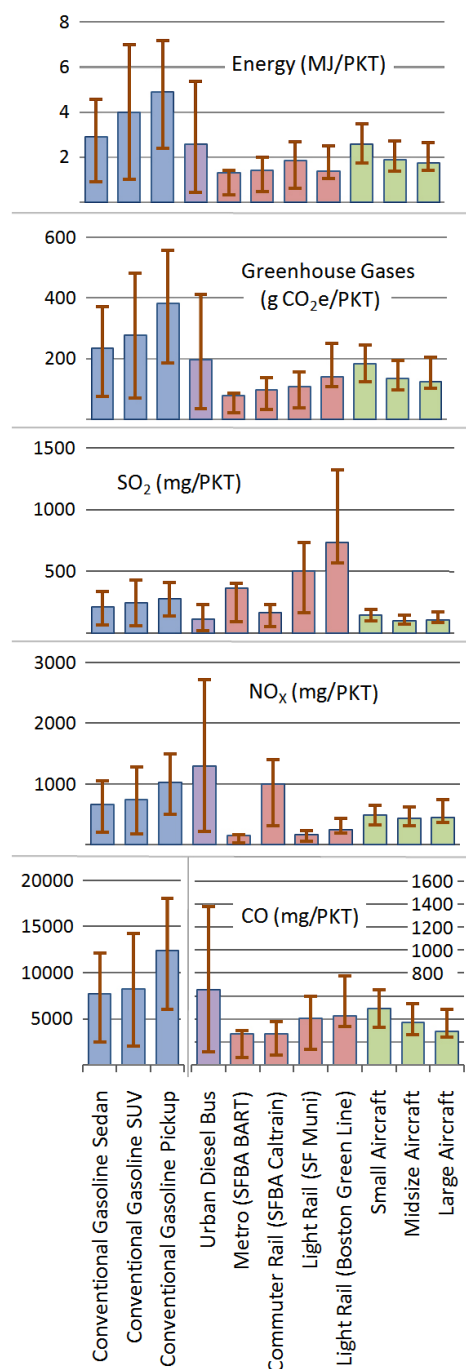
Figure 3. Occupancy sensitivity (Average occupancy and life-cycle performance is shown as the blue (autos), purple (bus), red (trains), and green (aircraft) bars. The maroon-colored line captures the range in per-PKT energy consumption and emissions at low and high occupancy).
