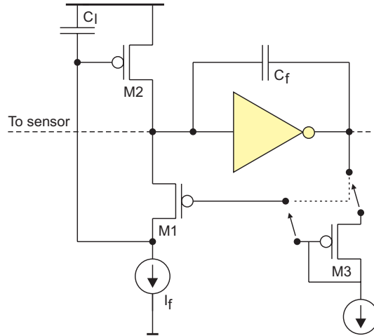
Figure 7. Charge preamplifier feedback circuit.
