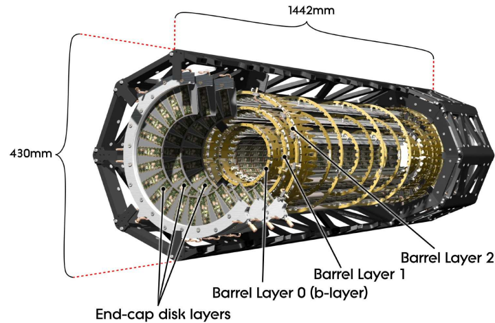
Figure 2. A schematic view of the active region of the pixel detector consisting of barrel and endcap layers.
