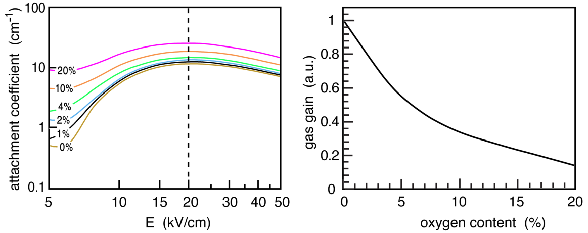
Figure 9. Left: electron attachment coefficient as a function of the electric field strength. Right: the gas gain as a function of the oxygen content.
