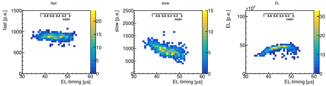
Figure 10. EL-timing dependence on the number of photons detected. From left to right, the three plots correspond to the fast component, slow component, and the EL signal. The drift electric field is applied at 6.6 V/cm/atm, and the EL one at 900 V/cm/atm.
