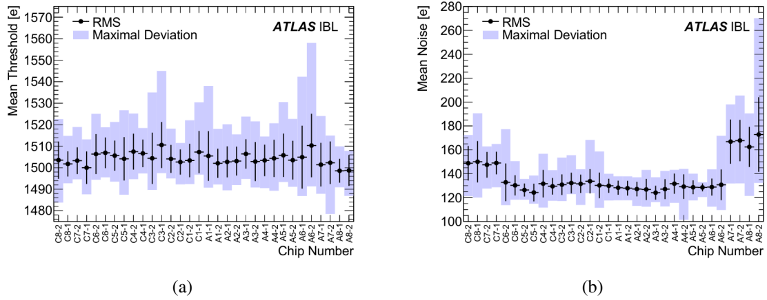
Figure 40. (a) Mean threshold and (b) mean noise (ENC) distributions for all 18 qualified staves as a function of the chip number (position) on the stove, for a 1500 e - threshold tuning at -12 °C . The error bars represent the RMS value accounting for the differences between staves whereas the solid colour describes the full range covered by data.
