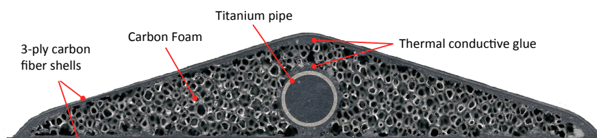
Figure 23. The transverse section of a bare stave.
