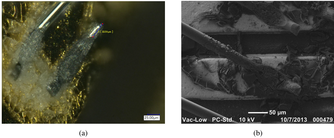
Figure 46. (a) White residue of corrosion on staves as observed under a microscope. (b) A Scanning Electron Microscopy (SEM) image of corroded wires and the corrosion residue at the foot of the bond.
