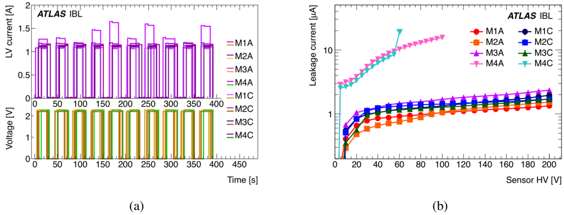
Figure 36. (a) LV cycles and (b) sensor I-V characteristics for the 8 DCS groups of stave ST12. The DCS granularity is a group of four read-out chips (two planar modules or four 3D modules).
