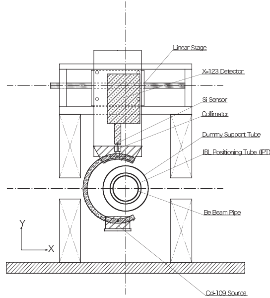
Figure 54. Beam pipe X-ray scanning equipment.
