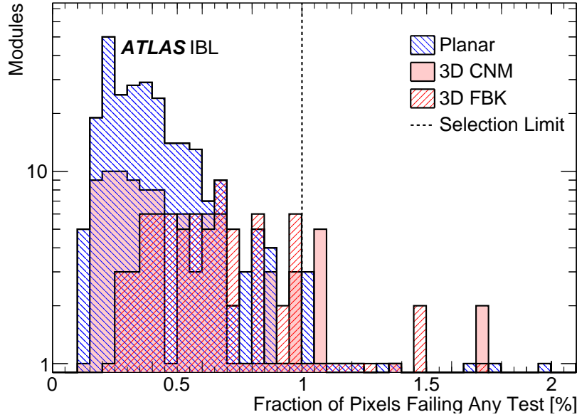
Figure 20. The distribution of the fraction of pixels failing in any test. Only modules otherwise accepted for stave loading are included. The modules are tuned to a 3000\text{ e}^- threshold, and 10 ToT counts for a charge injection of 16\text{ ke}^- , at a nominal operating temperature of -15^\circ\text{C} . A pixel is counted if it fails any one of the tests as described in the text. The selection limit is shown as a vertical line. Overflow entries are not shown.
