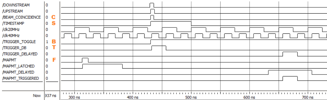
Figure 8. The DAQ system timing diagram showing the principal signals.
