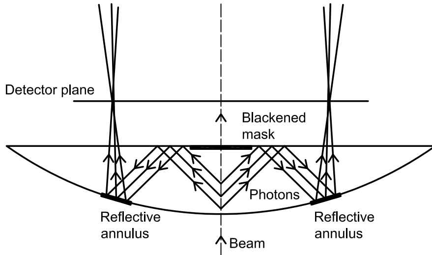
Figure 2. Schematic of the optical setup. Particles traverse the lens generating Cherenkov light, which is reflected at the flat surface and reflected and focused on the curved surface of the lens. Most rays converge at the position of the photon detectors.
