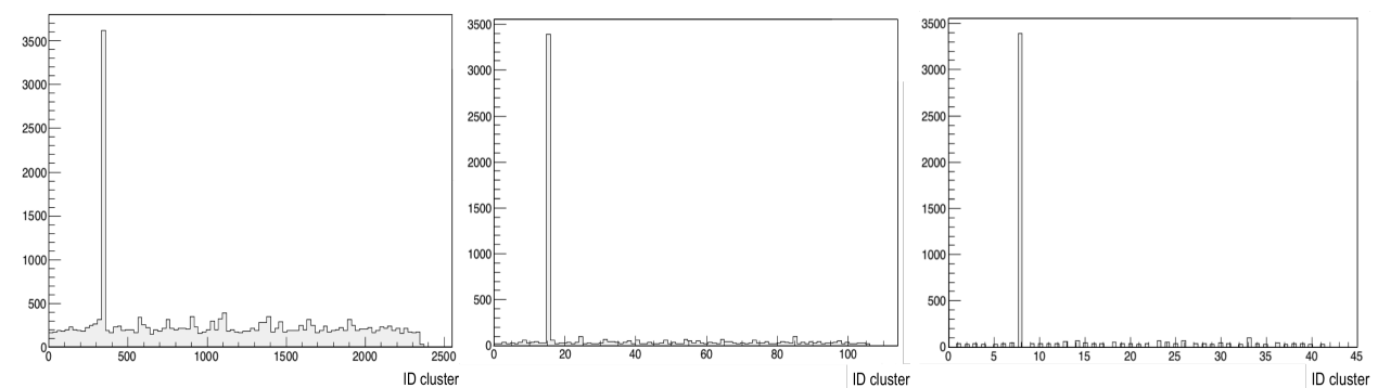
Figure 2. Results of the modified FOF algorithm applied on a dataset with high-Z material using a r_l = 5\text{ cm} and N_{min} equals to 5, 20, 30 points respectively.
