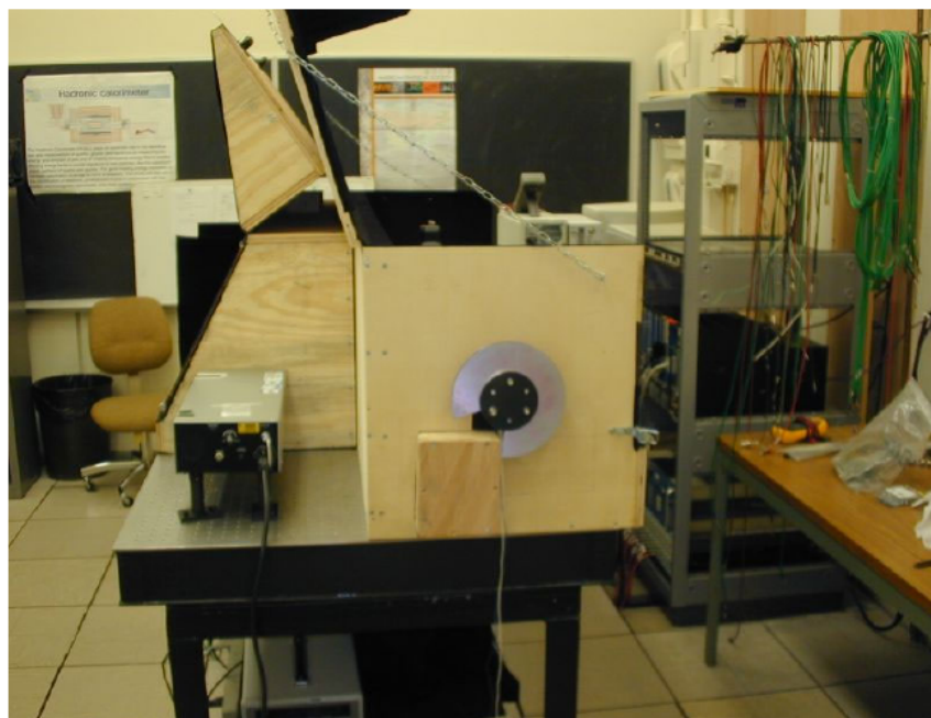
Figure 8. The University of Iowa PMT test station.
