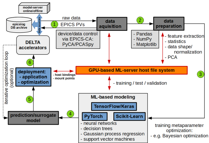
Figure 3. Concept of the EPICS/Python-based ML-workflow (steps 1 to 6). First, the ML-training data were collected from the accelerator facility (1). After data preparation (2), these data were used for offline model training (3) of surrogate injection models (4). Finally, the trained models, in turn, were loaded into the EPICS-based control system (5) and tested for injection optimization (6).
