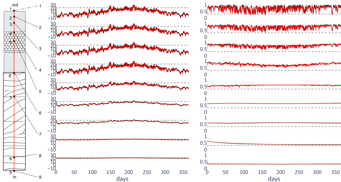
Figure 3. Simulated temperature [ ^{\circ}\text{C} ] (middle) and relative humidity [-] (right) from WUFI (black curves) and HAMOPY (red curves) in different section points (shown on the left) for TRY in OSLO, Norway.
