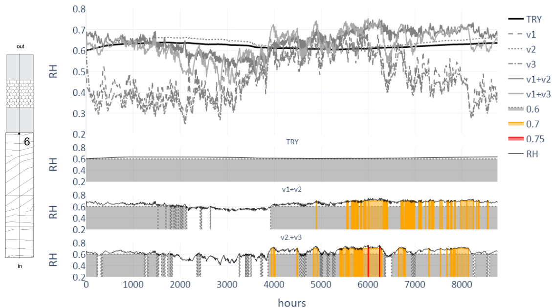
Figure 4. Simulated RH (top) for reference (TRY) and altered (v1,v2,v3,v1+v2,v2+v3) material properties, and corresponding mold growth risk periods for different potentially critical RH(0.6- grey, 0.7- yellow, 0.75 - red) in section point 6 for OSLO, Norway.
