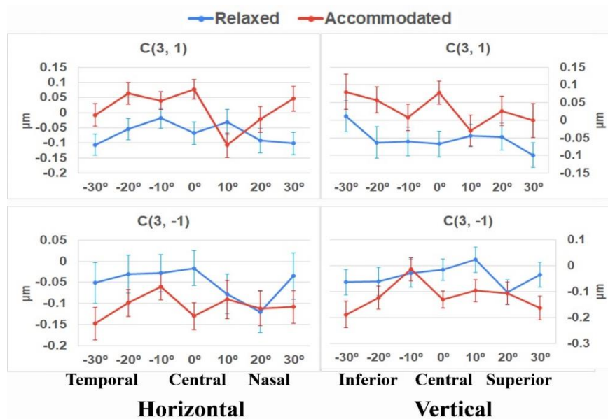
Figure 1. Plot of primary comas ( C_3^{-1} and C_3^1 ) in various points of fixation with and without accommodation in vertical and in horizontal meridian. The error bars represent the standard error of mean.
