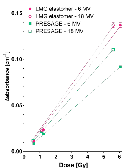
Figure 2. Difference of absorbance after and before irradiation against dose. Materials were irradiated whether at 6 MV (full symbols) or at 18 MV (unfilled symbols), with a dose rate of 5.3 Gy.min -1 . LMG elastomer (circles) and PRESAGE® (squares).
