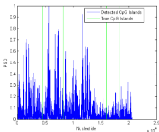
Figure 8. Result obtained using DWT method.
