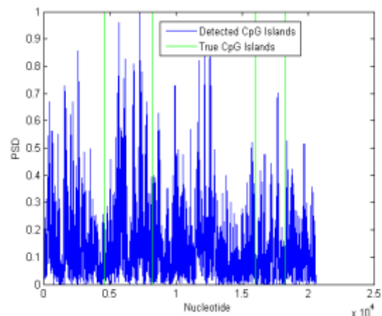
Figure 9. Result obtained using DWT using combination of 24 mappings of integer mapping method.
