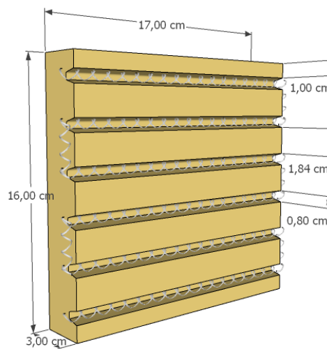
Figure 1. Rear side refractory design and dimensions
