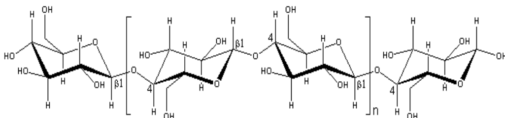
Figure 3. B (1-4) -D-glucoside linking chain on cellulose
