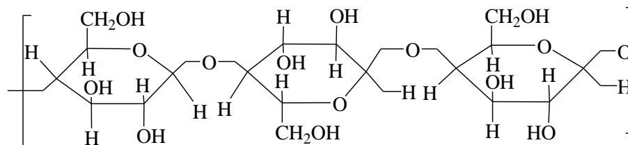
Figure 2. Cellulose structure
