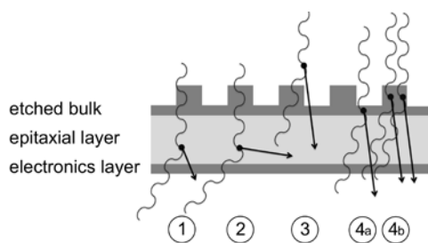
Figure 3. Compton scattering of a photon in the epitaxial layer (1, 2), in the air/LINAC (3), and in the grating etched in the bulk (4).
