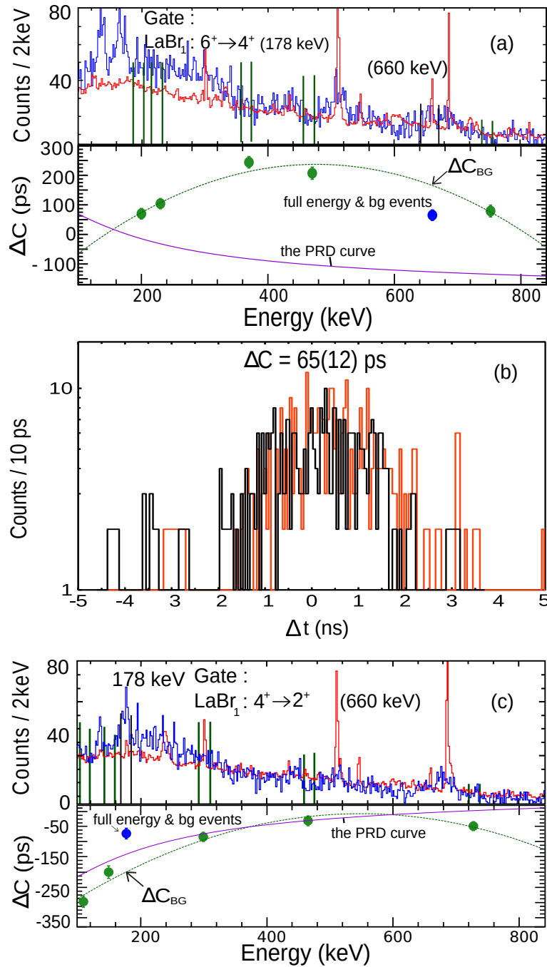
Figure 2. (Color online) The procedure of extracting the lifetime of the 4_1^+ state in ^{208}\text{Po} . (a) Double-gated spectra from LaBr (blue) detectors and HPGGe detectors (red) produced from triple coincidence data by imposing the indicated coincidence conditions (gates). Here, the gate on the first LaBr detector is set on the transition feeding the level of interest. The black lines indicate the gate, which was used to produce the time-difference spectra at the full energy peak (FEP) of the decay transition. The vertical green lines indicate the gates used to extract the time response of the background. The panel below presents the fitted time response of the background (dashed green line) with marked interpolated time response of the background; Together with the PRD curve (magenta line) and the obtained centroid difference (the blue circle). (b) Time-difference spectra for the 178- and 660-keV feeder-decay combination. (c) Same as (a) but the gate on the LaBr detectors is set on the decay transition.
