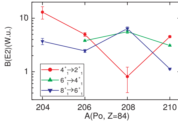
Figure 3. (Color online) The experimental B(E2) values for the seniority preserving transitions for the polonium isotopes. The result for the 4_1^+ \rightarrow 2_1^+ transitions in ^{208}\text{Po} is obtained in the present work. The results for ^{210}\text{Po} and the results for the 8_1^+ and 6_1^+ states in ^{208}\text{Po} are taken from Ref.[11]. The result for the 6_1^+ state in ^{206}\text{Po} is taken from Ref.[12]. The results for the 4_1^+ states in ^{206}\text{Po} and ^{204}\text{Po} are taken from Ref.[13].
