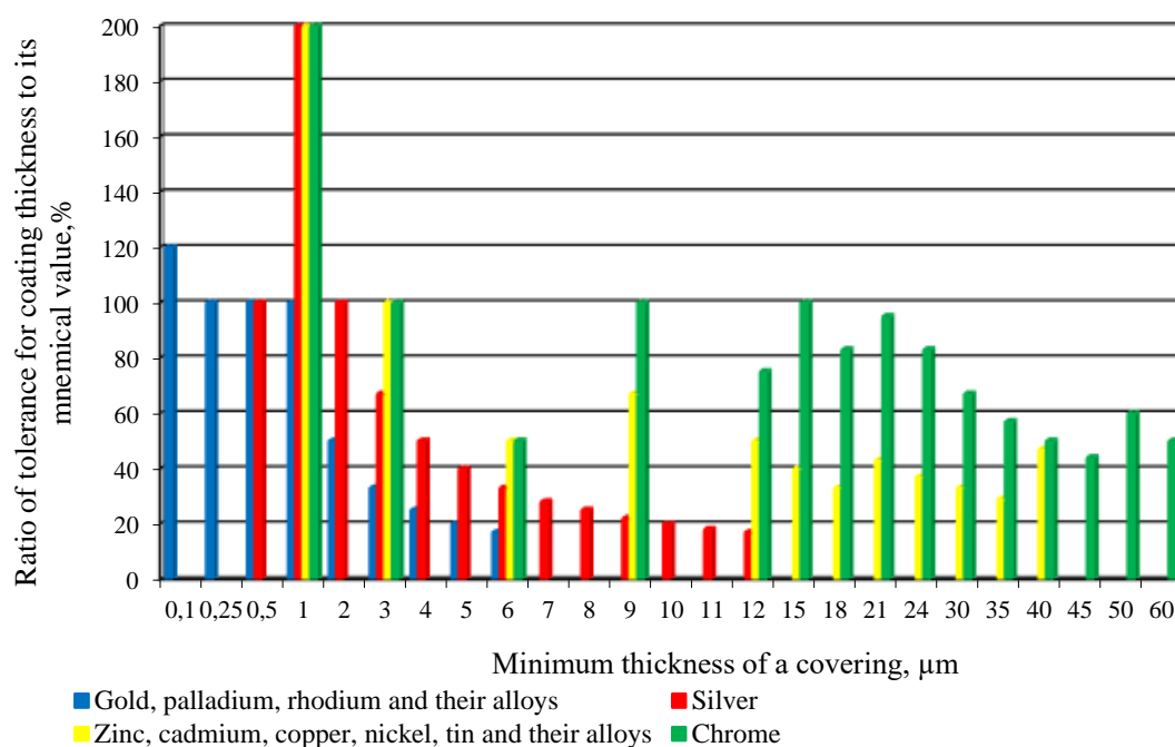
Figure 1. Ratio of tolerance to minimum thickness of coatings.
