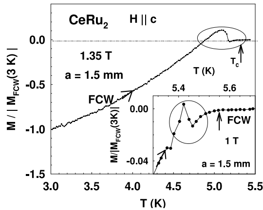
Figure 3. Plot of normalised magnetization vs. temperature for an applied field of 1.35 T and amplitude of vibration 1.5 mm
