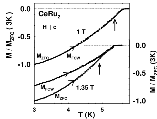
Figure 2. The isofield M-T data for 1 T and 1.35 T for both ZFC and FCW states for amplitude of sample vibration 0.3 mm.
