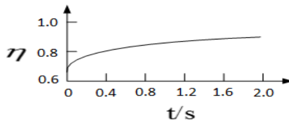
Figure 8. Charging waveform of supercapacitor
