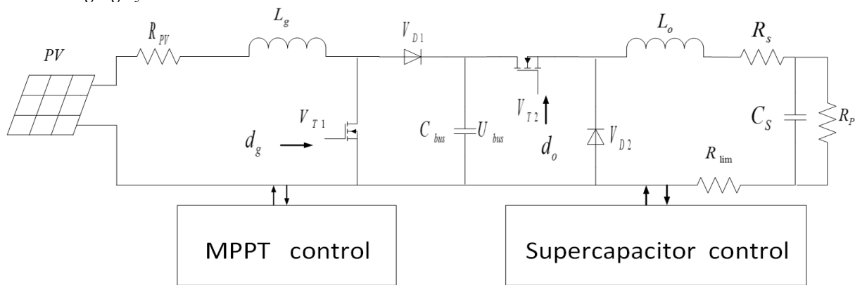
Figure 5. Structure diagram of charging system
