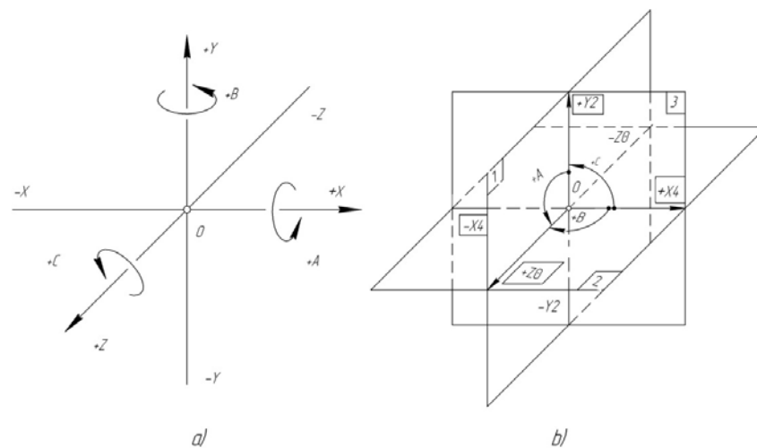
Figure 2. Right rectangular coordinate system: a) for metal-cutting machine tools according to ISO 841: 2001; b) for geometrical product specifications (alternative).
