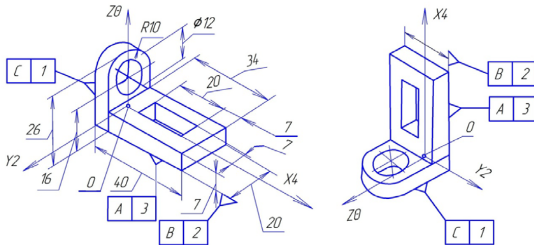
Figure 3. Natural position of the axis Z in the axonometric projection (a) and the unnatural one in the electronic model (b).
