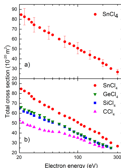
Figure 1. a) Present experimental total cross section (TCS) for the electron scattering from \text{SnCl}_4 and b) its comparison with TCSs for \text{CCl}_4 [2], \text{SiCl}_4 [3] and \text{GeCl}_4 [4] molecules. Error bars correspond to overall experimental uncertainties.
